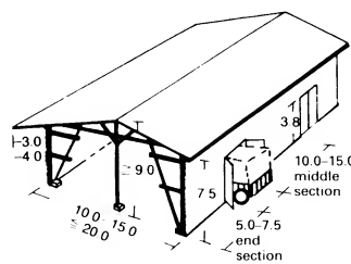
⑥ Barn with transverse aisles
